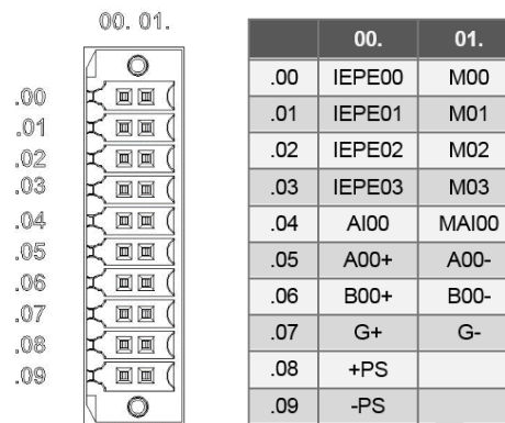
Fig 48. Module connector and pinout.
