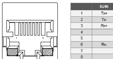
Fig 9. ETHERNET Connector.
