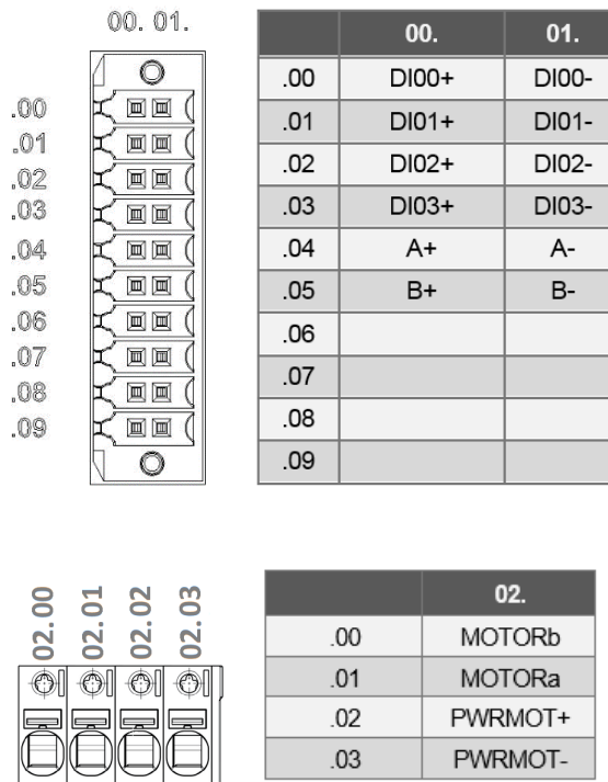
Fig 45. Motor module connector and pinout.
