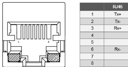
Fig 7. PROFINET RT S Connector.
