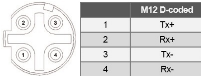
Fig 8. ETHERNET Connector.
