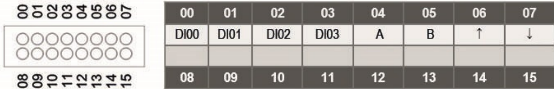
Fig 44. Module indication LEDs.
